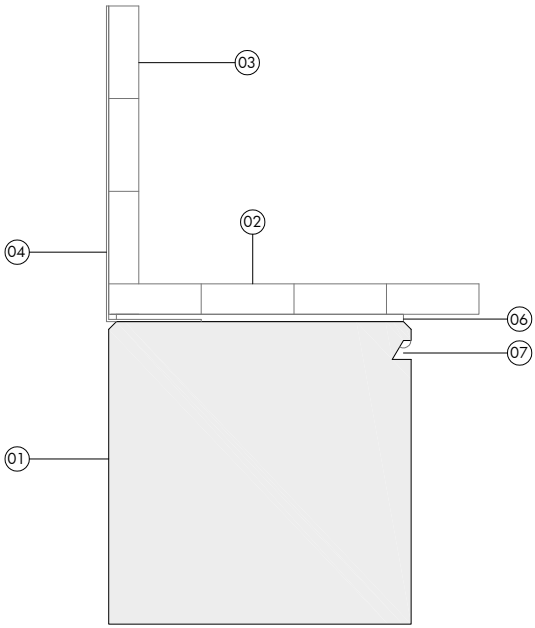
Detall 2 banc tram 2 e:1/10
