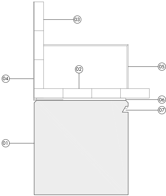
Detall 1 banc tram 1 e:1/10
